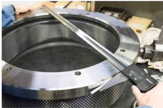
▲ Outer Diameter Measurement
